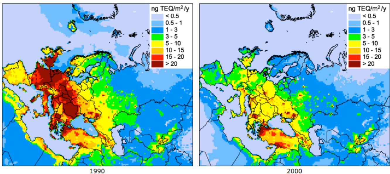
Spatial distribution of PCDD/F deposition , ng TEQ/m 2 /y
